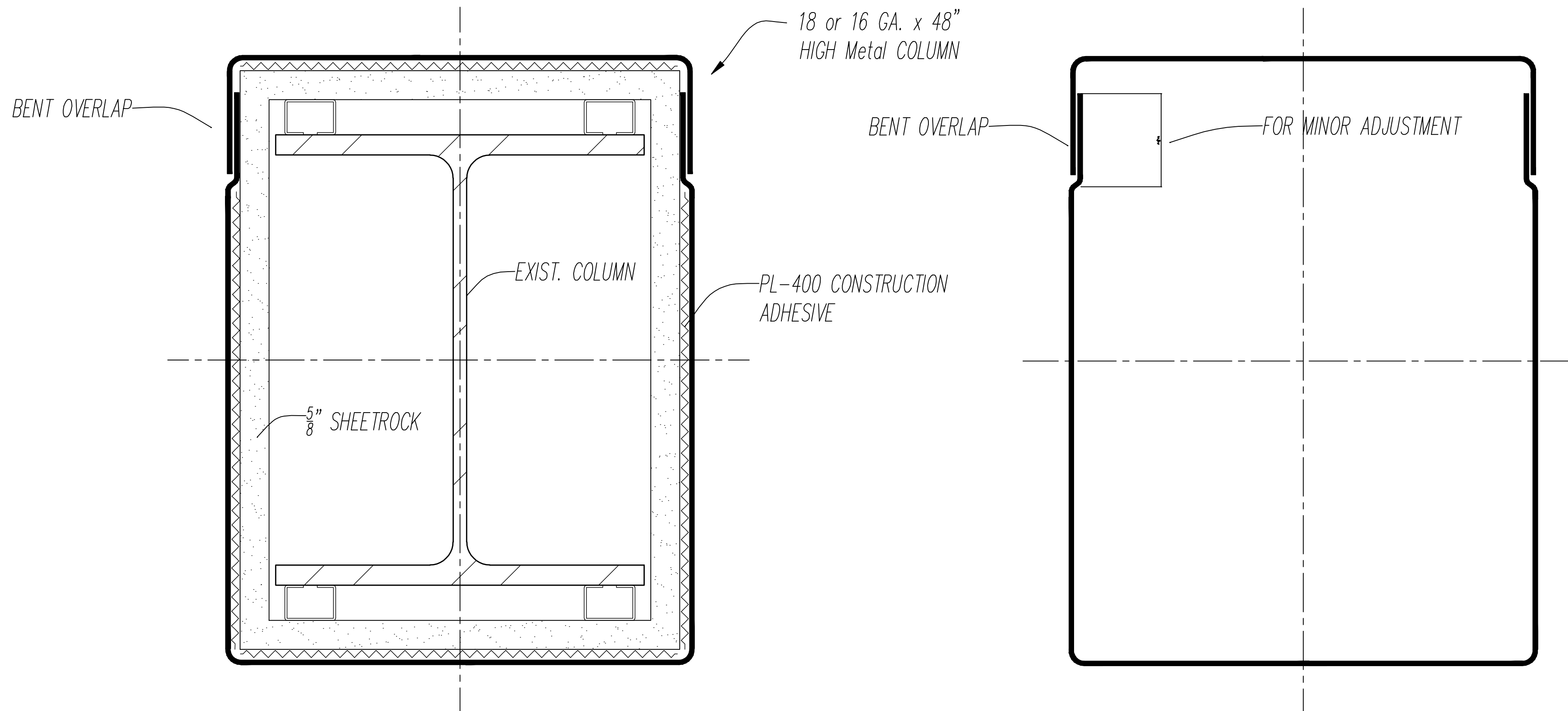
Guards Column Typ. 48" High TYPICAL SECTION THRU EXIST. COLUMN PART NO. MTGC48
